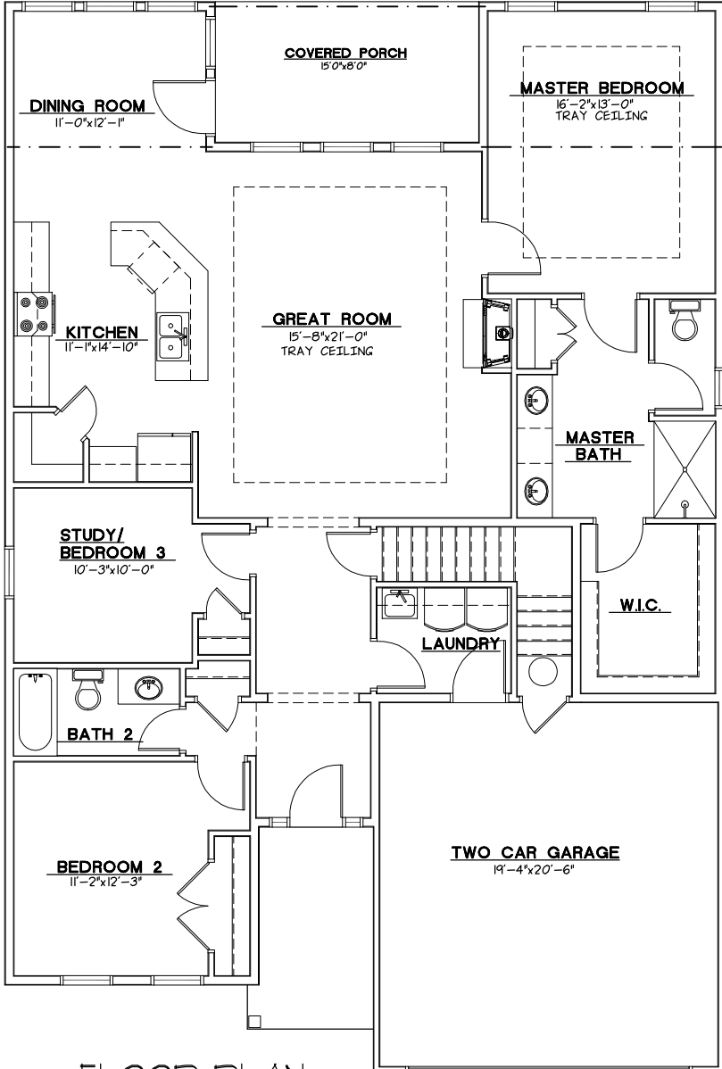
FLOOR PLAN (1,743 Sq. Ft. Living Space)
